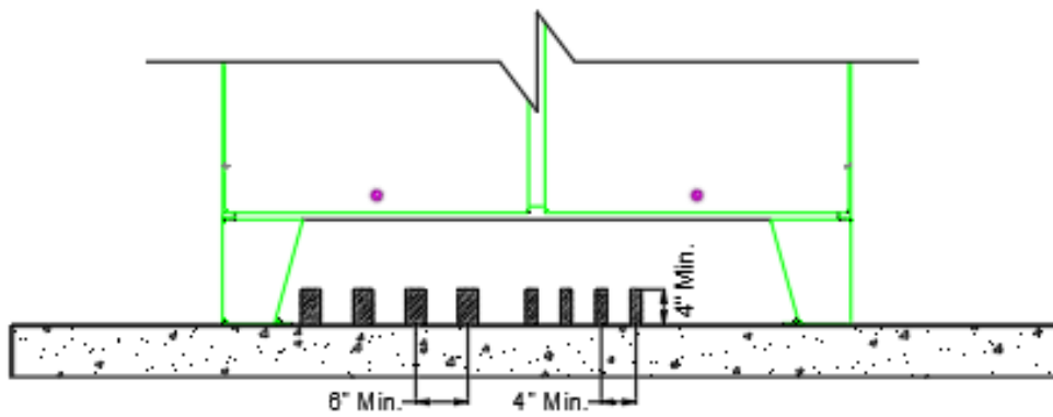
Conduit and Pad Layout for 1-4 Circuit Panel
